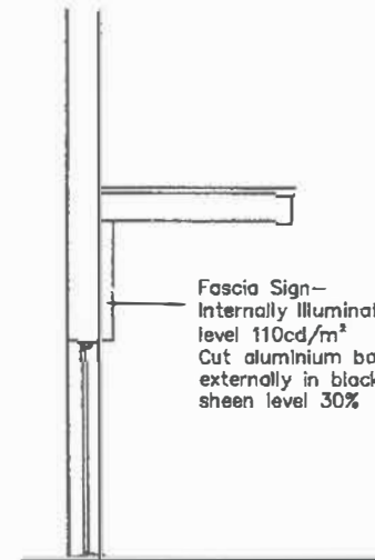
Proposed Section @1:50
